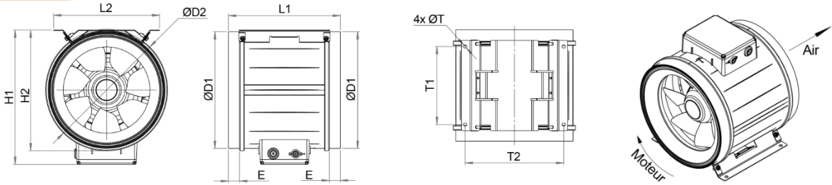
Dimensions (mm)
