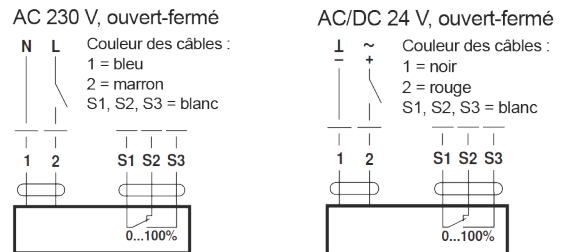
Câblage LF230S
